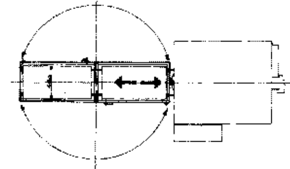
ROTATING 2 POSITIONS LOADING TABLE
